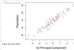
Fig 6.16 from ISLR
