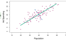
Fig 6.14 from ISLR
