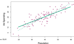
Fig 6.21 from ISLR
